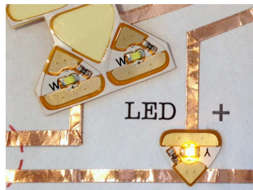
Figure 1. Illuminated LED circuit sticker
