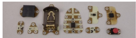
Figure 2: Circuit stickers. From left: generic 0805, piezo sounder, LED, coin-cell battery holder, 555 timer, hall-effect sensor, accelerometer, push button.
