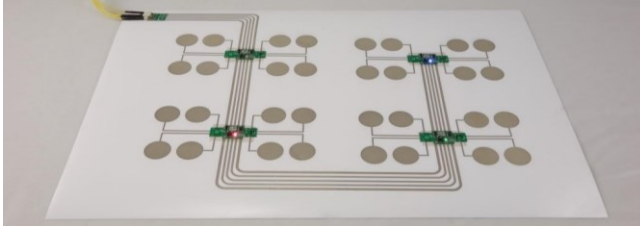
Figure 7: I2C bus-based design with distributed touch sensors and color LEDs. An I2C bus master connected by the yellow wires (top left) polls the touch sensors and controls the LEDs.
